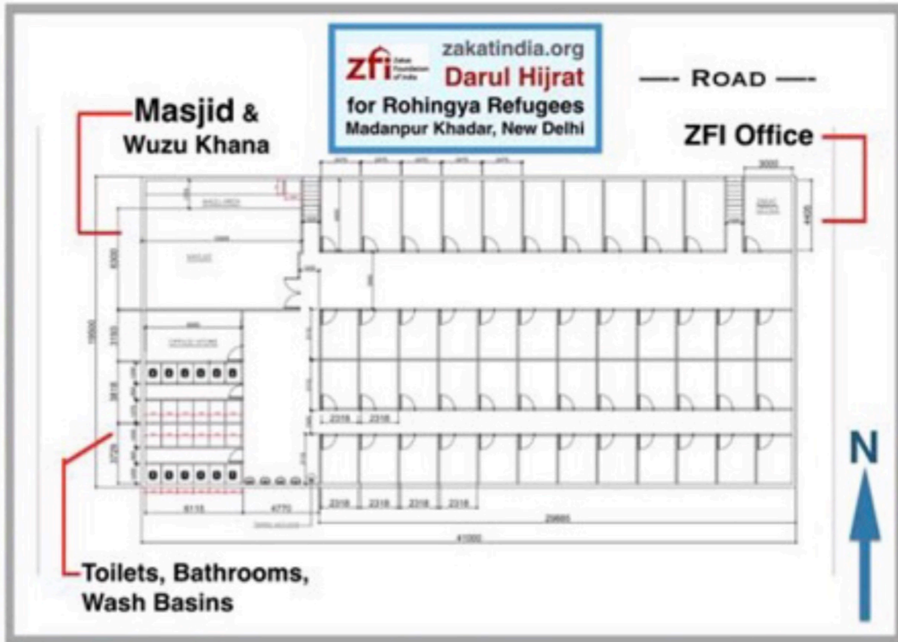
ZFI'S REHABILITATION PLAN (after fire on April 15, 2018)
